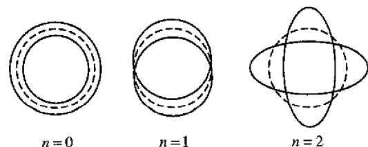
Fig. 2 Circumferential mode shapes according to the circumferential mode number ( n )
