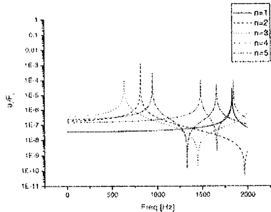
Fig. 4 A typical receptance of the shell according to the order of n circumferential mode
